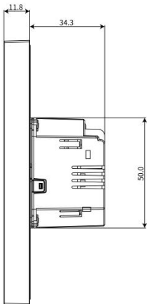
② RIGHT VIEW
