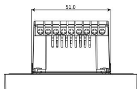
⑥ TOP VIEW
