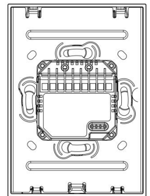
④ BACK VIEW
