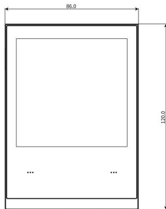
① FRONT VIEW
