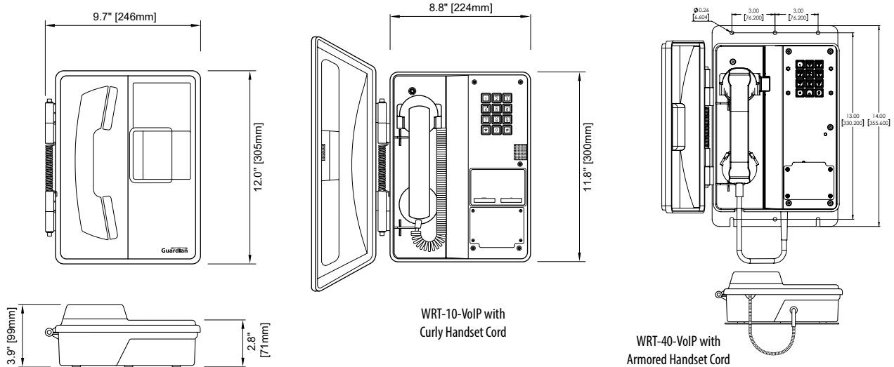
WRT-V SERIES Weather Resistant VoIP Ringdown Telephones
