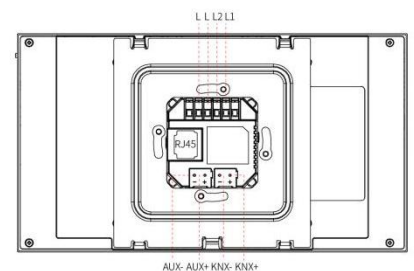
4 BACK VIEW
