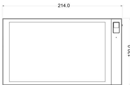
1 FRONT VIEW
