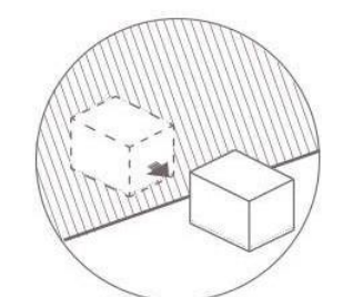
Object Removed
