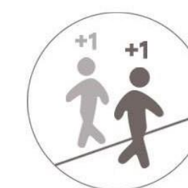
People Counting
