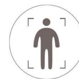
Human Detection
